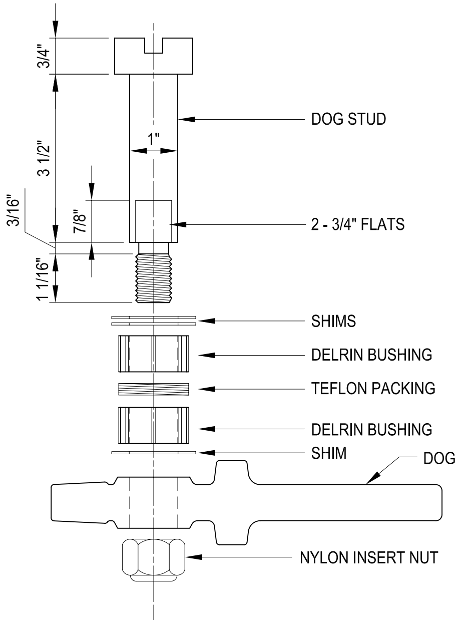
SIDE VIEW
